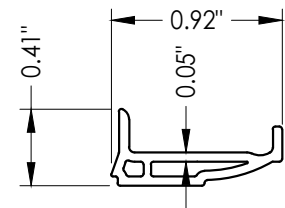
9 GLAZING BEAD
