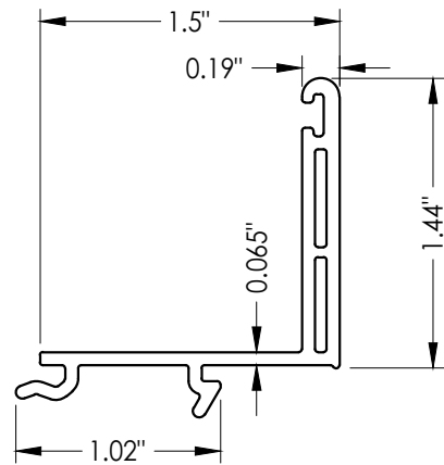
4 SILL ADAPTER
