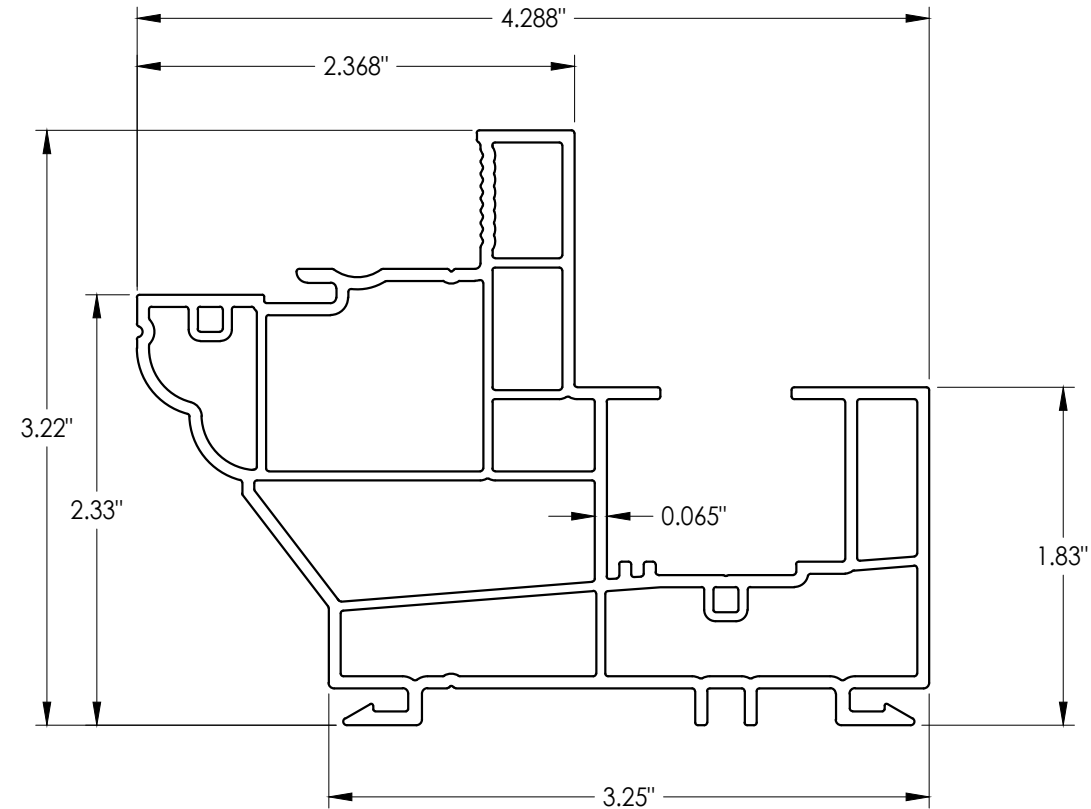
1 FRAME
