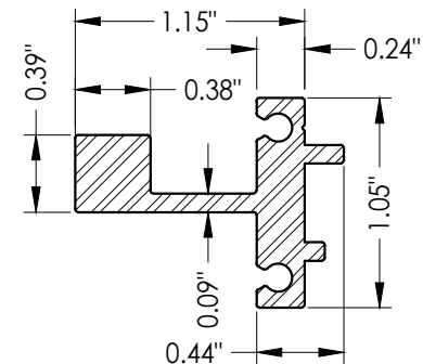
12 REINFORCEMENT
