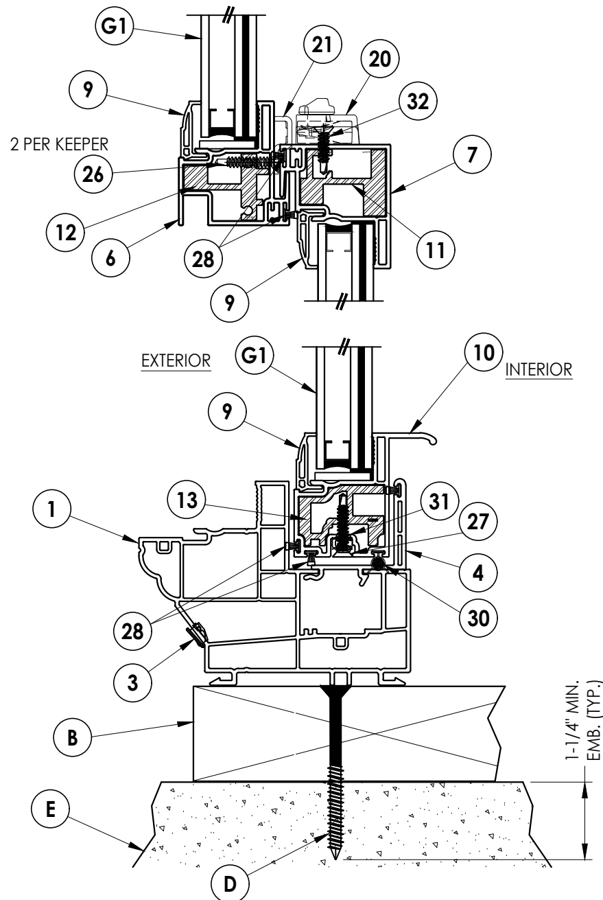
4 4 VERTICAL CROSS SECTION 2X Buck Construction
