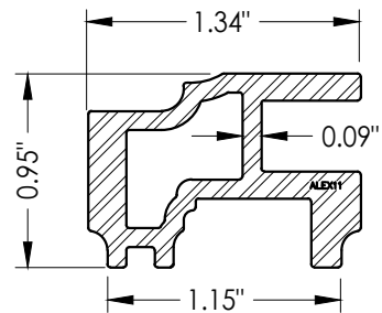
13 REINFORCEMENT
