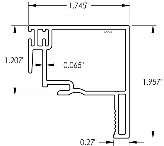
7 LOCK RAIL
