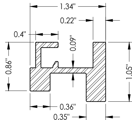
11 REINFORCEMENT
