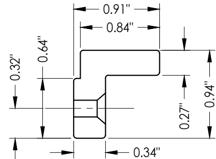
24 TILT LATCH BLOCK
